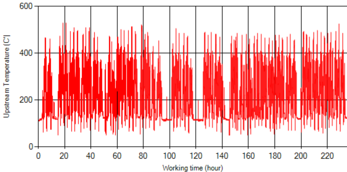
Figure 7- Temperature vs. working hours
